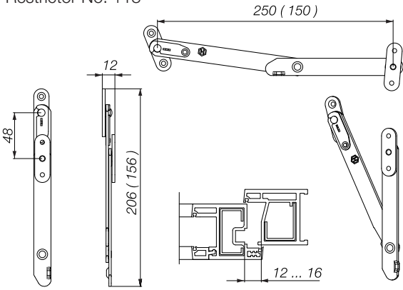
Restrictor No. 113
