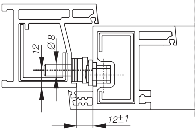
Vertical section KSP on the PVC window
